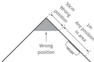
Slanting installation position
