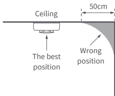
Ceiling installation position
